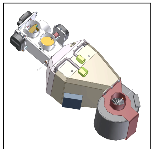
TAT custom-tailored ECS cabin climatisationair mixing chamber including vapor cycle air conditioning evaporator
